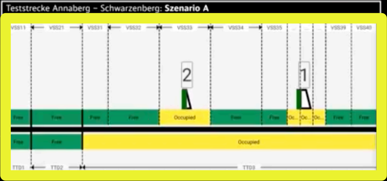
ProB running in real-time animating a formal B model of the Hybrid-Level 3 principles developed by a team from the University of Düsseldorf and Thales with support from ClearSy
